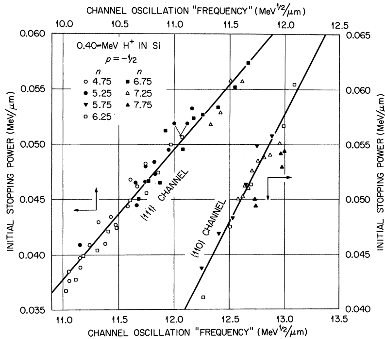
FIG. 4. Dependence of the initial stopping power of 0.4-MeV protons on their oscillation frequencies in the \{111\} and \{110\} channels of thin silicon crystals.
