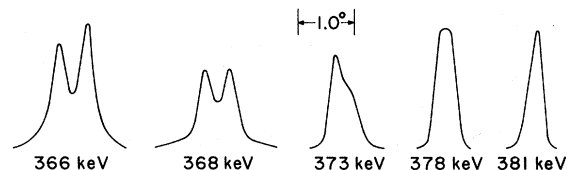
FIG. 3. Angular distributions observed for 0.4-MeV protons transmitted through the {111} channels of a 0.53- \mu\text{m} Si crystal. The {111} plane lies near the centroid of each distribution.
